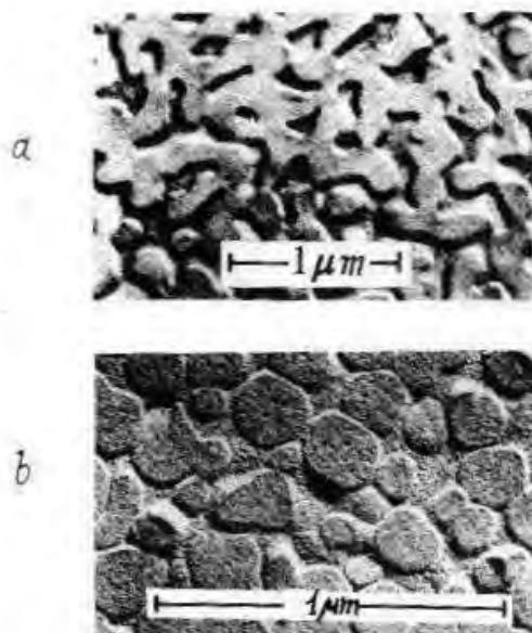
Fig. 2 In sharp contrast with the hypothetical calculations based on Zachariasen's random network theory, is the direct TEM evidence. Shown are some examples of binary and ternary glasses, some quenched, some heat-treated which clearly show actual phase-separation. One can confidently assume that in many if not most glasses and in many liquids, structural (-composition) fluctuations must exist as precursors to such phase separation (after Mazurin and Porai-koshits) [11].
