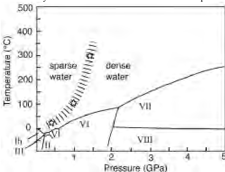
Fig. 6 The paper by Kawamoto et al. shows a projection of at least two water structures into the stable liquid water region exactly analogous to Fig. 4's experimental data on several liquid structures in liquid sulfur some 35 years earlier [22].
