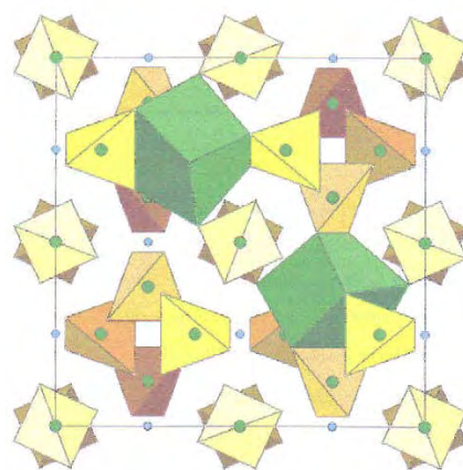
Fig. 11 The final “molecule” in the structure, the eight coordinated, or cornered, green cubes, is added, and knitted into a fixed position. The relationship of the atoms and polyhedra within the outlined (unit cell)
